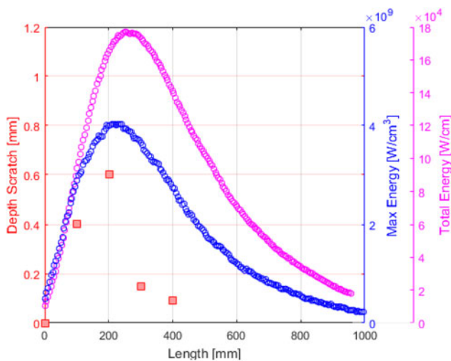
Figure 11. 3D topography results for the scratch at \eta_y = -5 mm on CuCD blocks. The absolute value of the depth is plotted, together with the total energy and the energy density (courtesy of E. Skordis) for shot#3 in Table 4.
